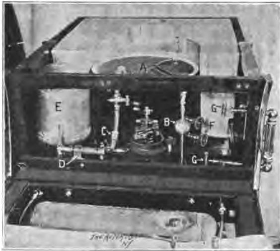
FIG. 261.—The Engine, Boiler and Attachments of the "Reading" Steam Carriage, shown in position. A is the fuel feed tube shown passing down through one of the boiler flues; B, valve for turning off fuel supply from the burner; C, expansion joint between the boiler and engine, permitting of some swinging movements; D, auxiliary hand feed pump; E, try cocks tapped into the boiler shell; G, G, hand valves of the water glass. The fuel tank is shown in the foreground, directly beneath the floor at the driver's feet.
